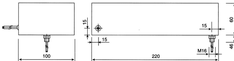
Note: XL-384 screw size = M 24 x 50 Fig1
